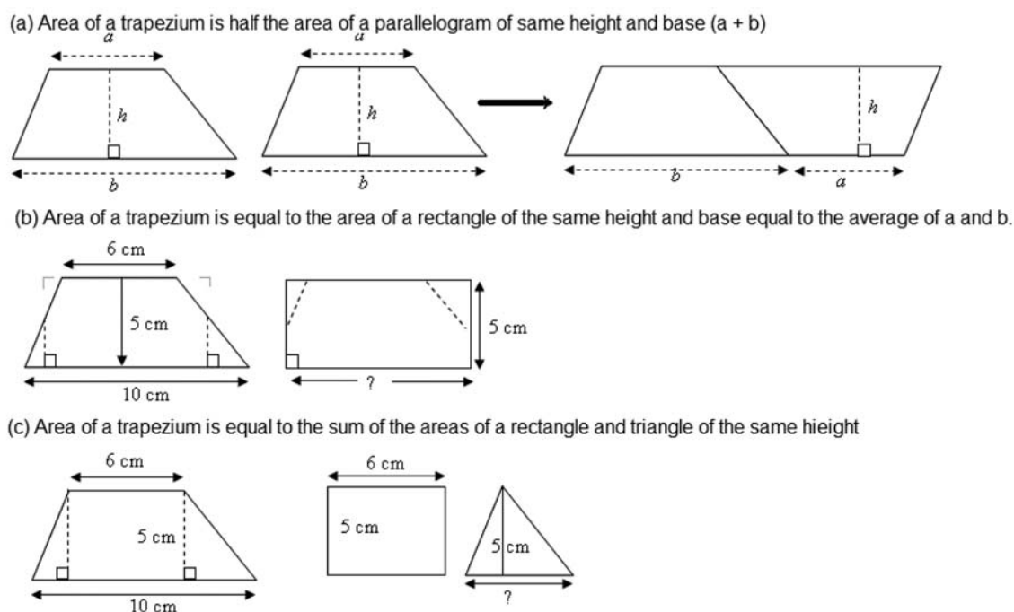
Figure 2. Three derivations of the area of a trapezium.
